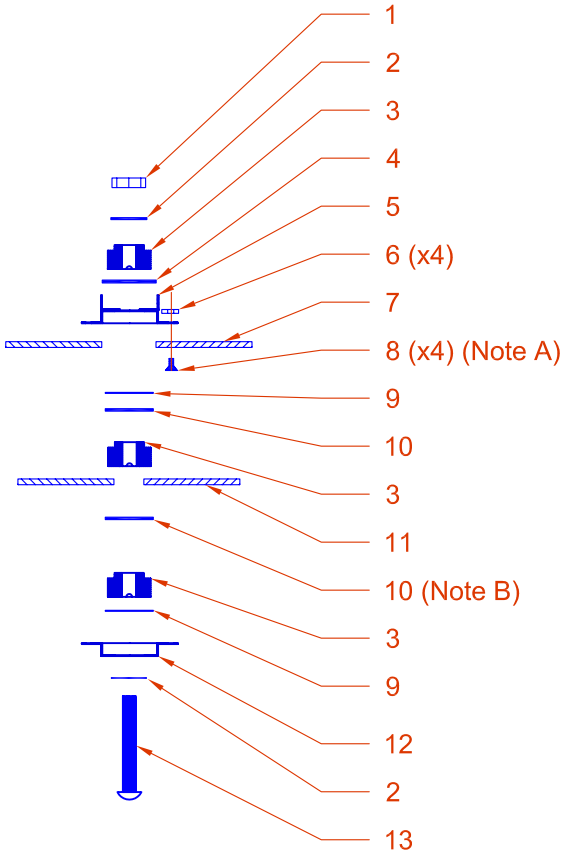
Grid Assembly Stack (Collimated)
